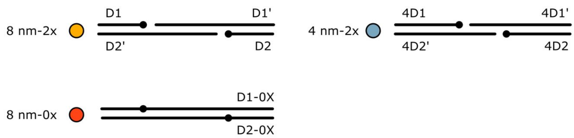
Supplementary Figure 1 Schematic representation of the three designs used in this work. The sequences of labelled strands can be found in Supplementary Table 1.
