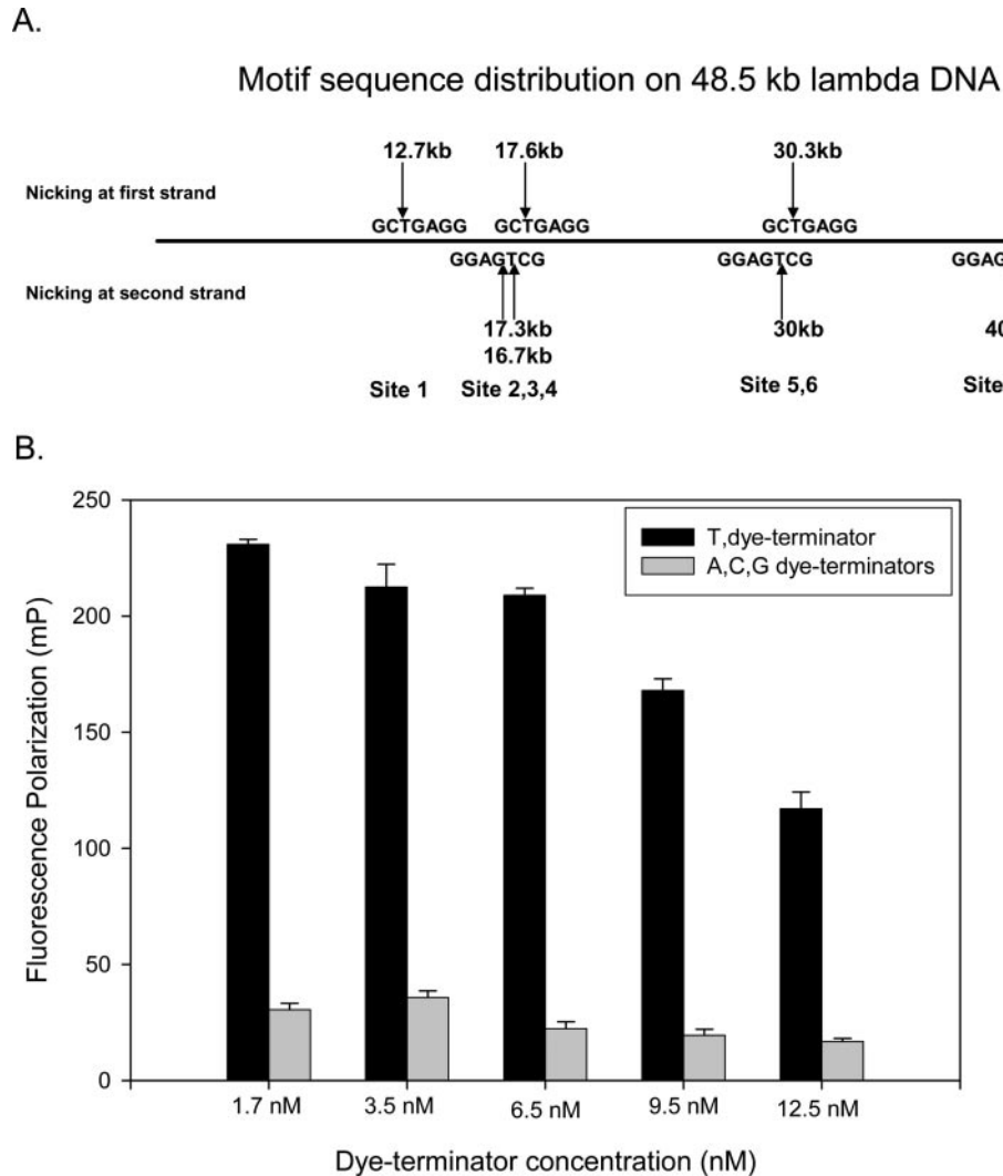
Figure 3. The sequence motif distribution on lambda-DNA and nick-labeling. (A) The sequence motif distribution on lambda-DNA. There are seven Nb.BbvC I sites along the 48.5 kb lambda-DNA. (B) The results of titration of dye-terminator incorporation for 1 nM lambda-DNA after nicking. Only the T-dye-terminator was incorporated at the entire range of terminator concentrations. As monitored by fluorescence polarization, where high FP values correspond to high proportion of incorporated dye-terminator in the reaction, dye-terminator incorporation was complete at \leq 6.5 nM of dye-terminators, showing that labeling occurred at all seven Nb.BbvC I sites.
